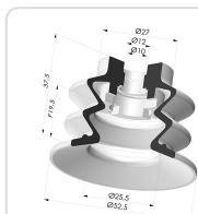
Bellows Suction Cup 2.5 folds Series 96, Ø 52 mm
