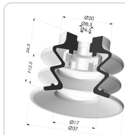
Bellows Suction Cup 2.5 folds Series 96, Ø 35 mm
