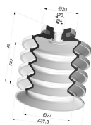
Bellows Suction Cup 4.5 folds Series 92, Ø 40 mm
