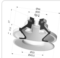
Bellows Suction Cup 1.5 folds Series 91, Ø 40 mm
