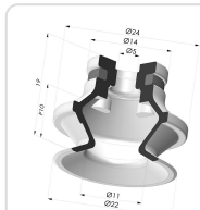
Bellows Suction Cup 1.5 folds Series 91, Ø 20 mm
