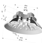
Flat Suction Cup Series 94, Ø 100 mm
