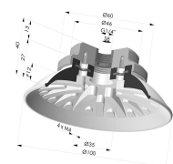
Flat Suction Cup Series 94, Ø 100 mm
