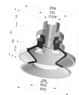
Bellows Suction Cup 1.5 folds Series 91, Ø 50 mm
