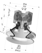
Bellows Suction Cup 1.5 folds Series 91, Ø 40 mm
