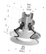
Bellows Suction Cup 1.5 folds Series 91, Ø 40 mm
