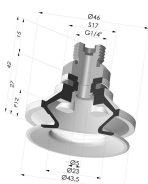
Bellows Suction Cup 1.5 folds Series 91, Ø 40 mm
