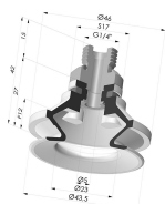
Bellows Suction Cup 1.5 folds Series 91, Ø 40 mm
