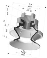
Bellows Suction Cup 1.5 folds Series 91, Ø 35 mm
