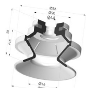
Variant reference: 91 31MNT A • Color: Bordeaux • Matter: Non-staining material • Shore Hardness: SH60
