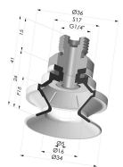
Bellows Suction Cup 1.5 folds Series 91, Ø 35 mm
