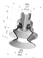
Bellows Suction Cup 1.5 folds Series 91, Ø 35 mm
