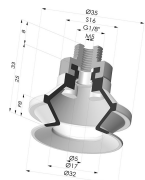
Bellows Suction Cup 1.5 folds Series 91, Ø 30 mm
