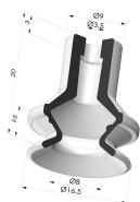
Bellows Suction Cup 1.5 folds Series 91, Ø 16 mm
