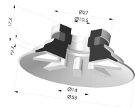
Flat Suction Cup Series 90, Ø 50 mm
