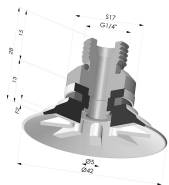
Flat Suction Cup Series 90, Ø 40 mm
