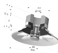
Flat Suction Cup Series 90, Ø 40 mm
