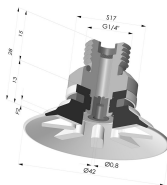
Flat Suction Cup Series 90, Ø 40 mm
