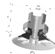
Flat Suction Cup Series 90, Ø 40 mm
