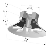
Flat Suction Cup Series 90, Ø 40 mm
