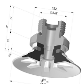
Flat Suction Cup Series 90, Ø 40 mm
