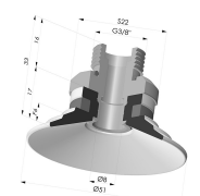
Flat Suction Cup Series 9, Ø 50 mm
