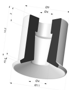
Flat Suction Cup Series 9, Ø 11 mm
