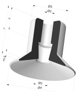
Flat Suction Cup Series 9, Ø 9 mm
