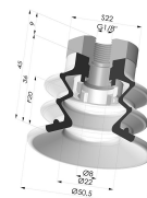
Bellows Suction Cup 2.5 folds Series 96C, Ø 50 mm
