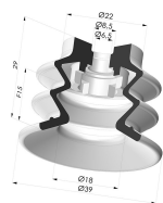
Bellows Suction Cup 2.5 folds Series 96C, Ø 40 mm
