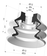
Bellows Suction Cup 2.5 folds Series 96C, 20 mm Ø
