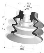
Bellows Suction Cup 2.5 folds Series 96C, 20 mm Ø
